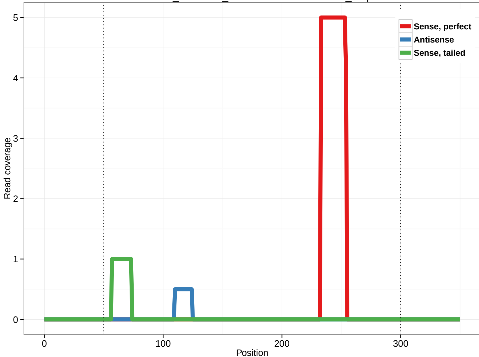
ornAna1_ensGene_ENSOANT00000001110_7.3p
