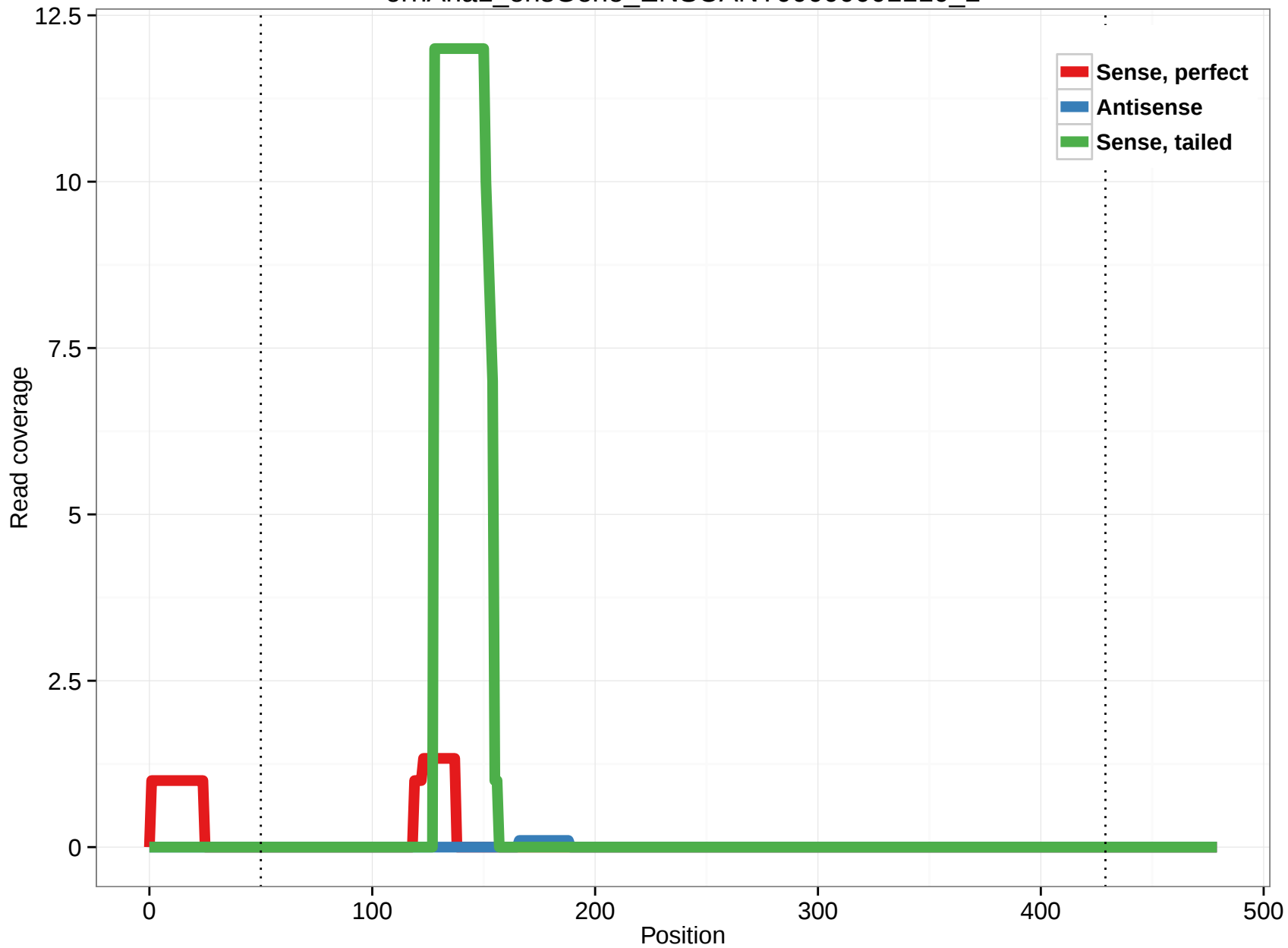
ornAna1_ensGene_ENSOANT00000001110_2
