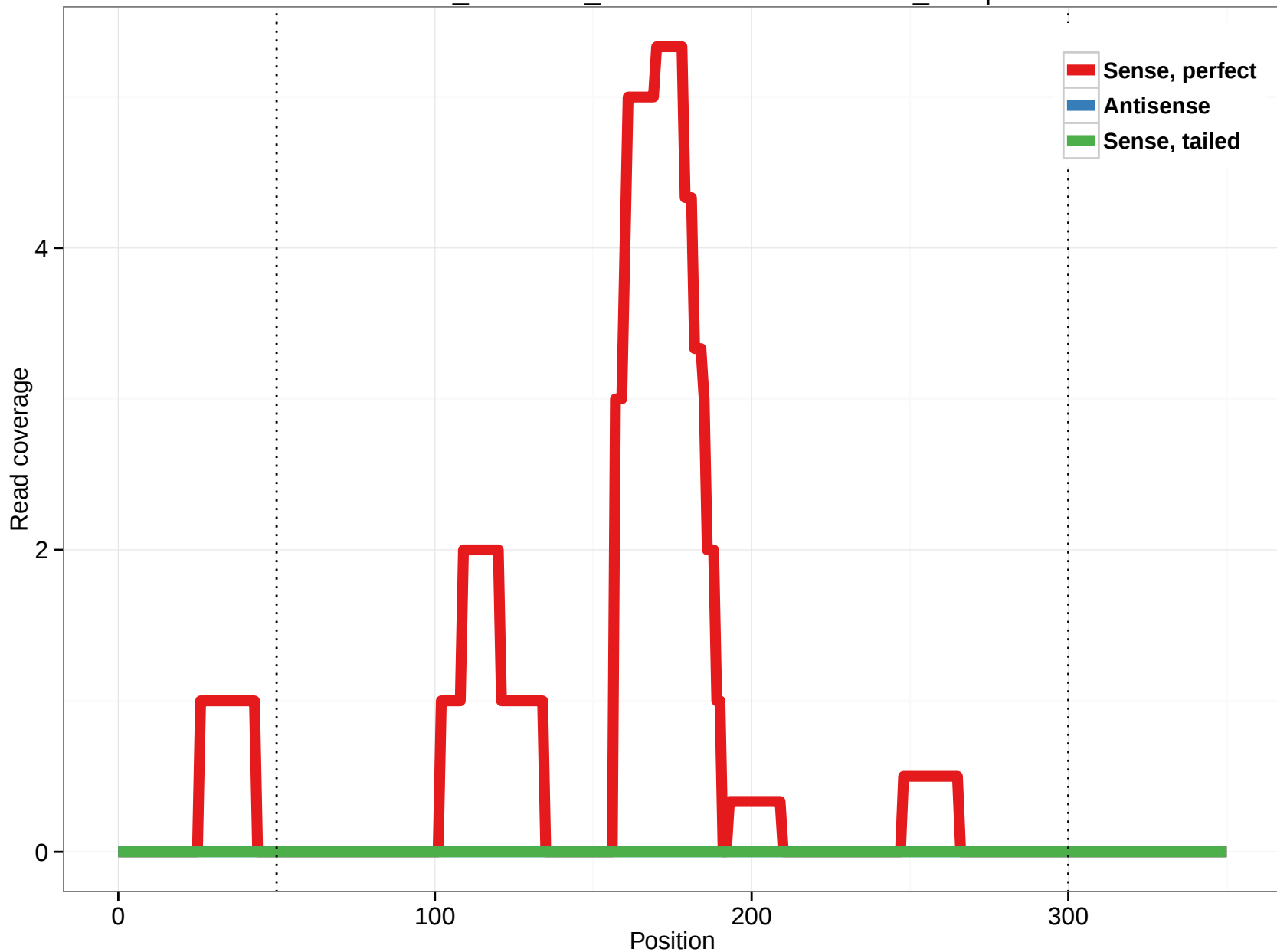
ornAna1_ensGene_ENSOANT00000001110_14.5p
