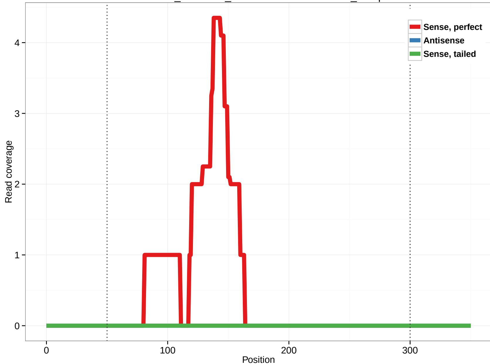
ornAna1_ensGene_ENSOANT00000001082_16.3p
