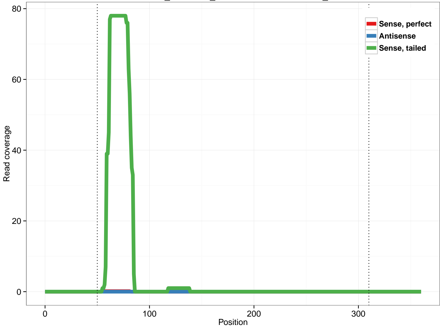
ornAna1_ensGene_ENSOANT00000001023_11
