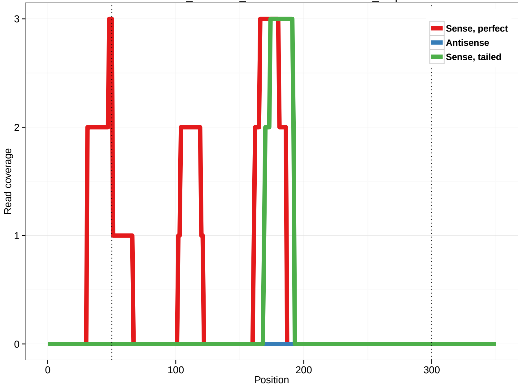
ornAna1_ensGene_ENSOANT00000001021_2.3p
