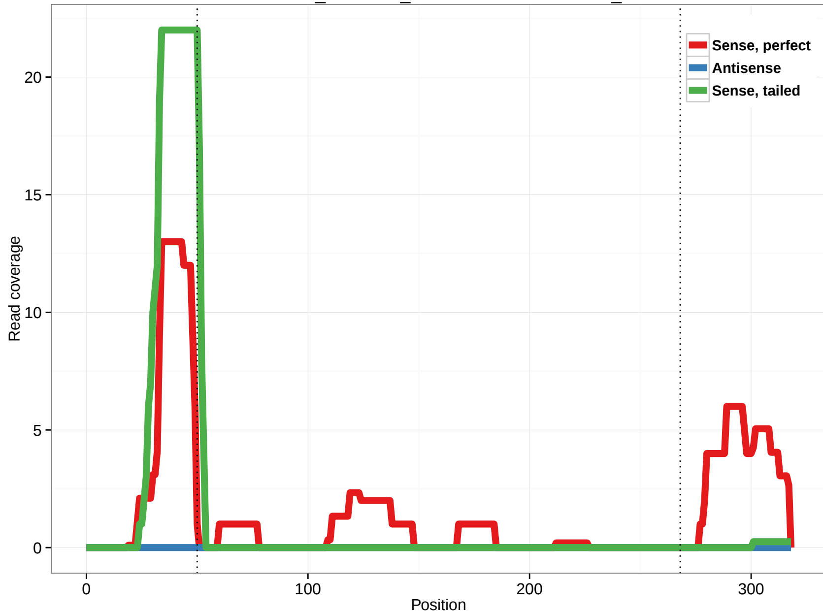
ornAna1_ensGene_ENSOANT00000001021_1
