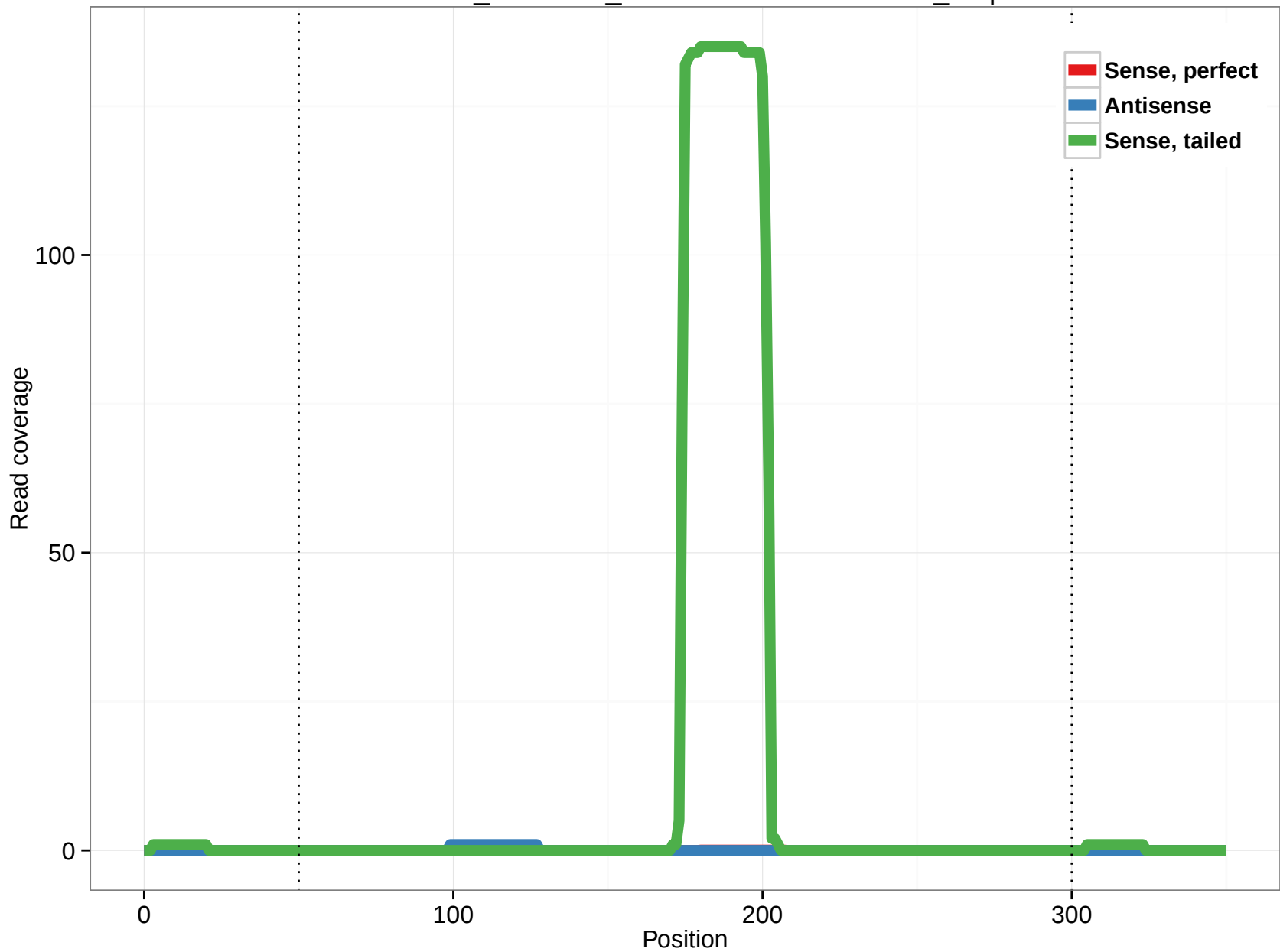
ornAna1_ensGene_ENSOANT00000001006_3.5p
