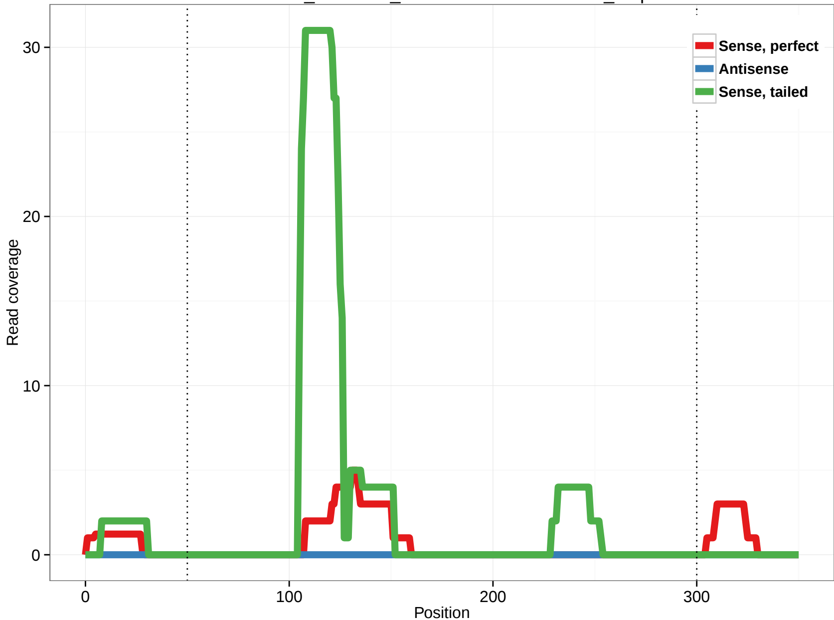
ornAna1_ensGene_ENSOANT00000000998_1.3p
