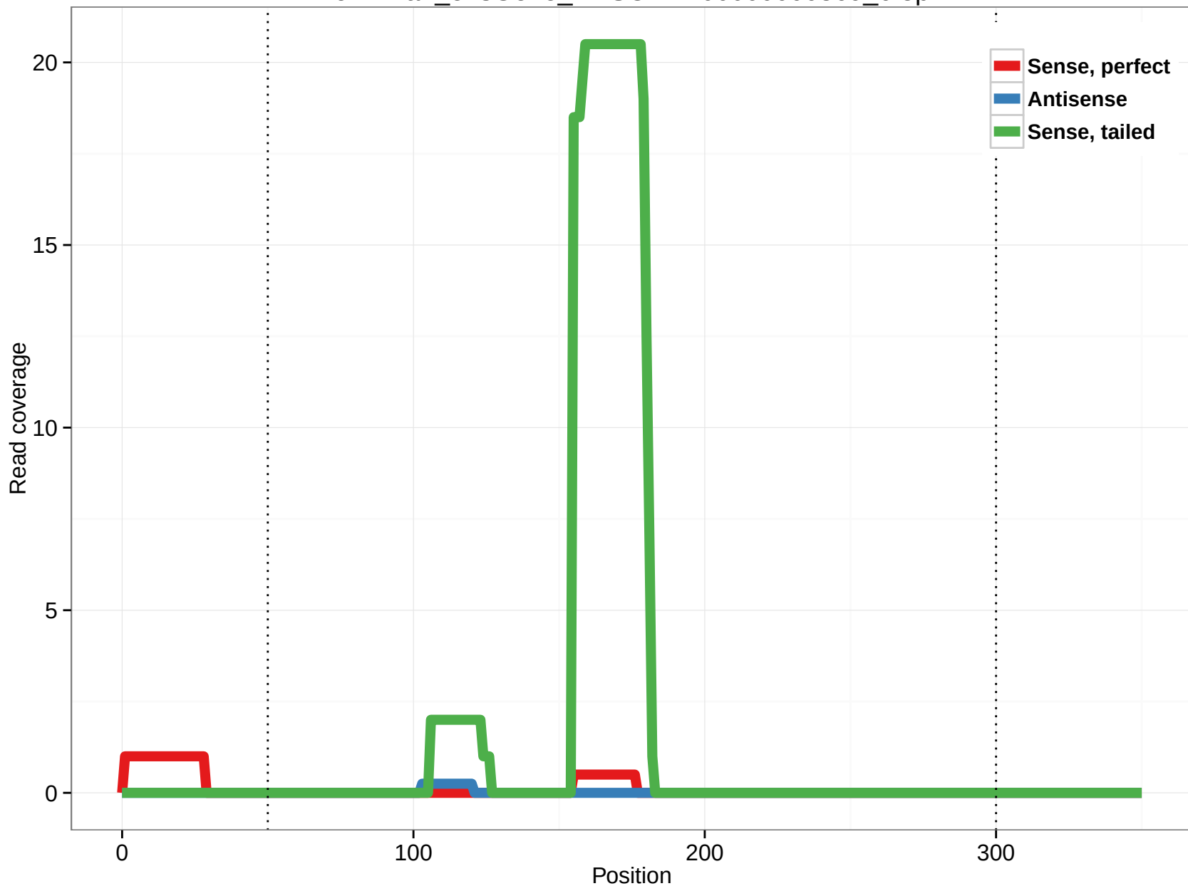
ornAna1_ensGene_ENSOANT00000000869_6.5p
