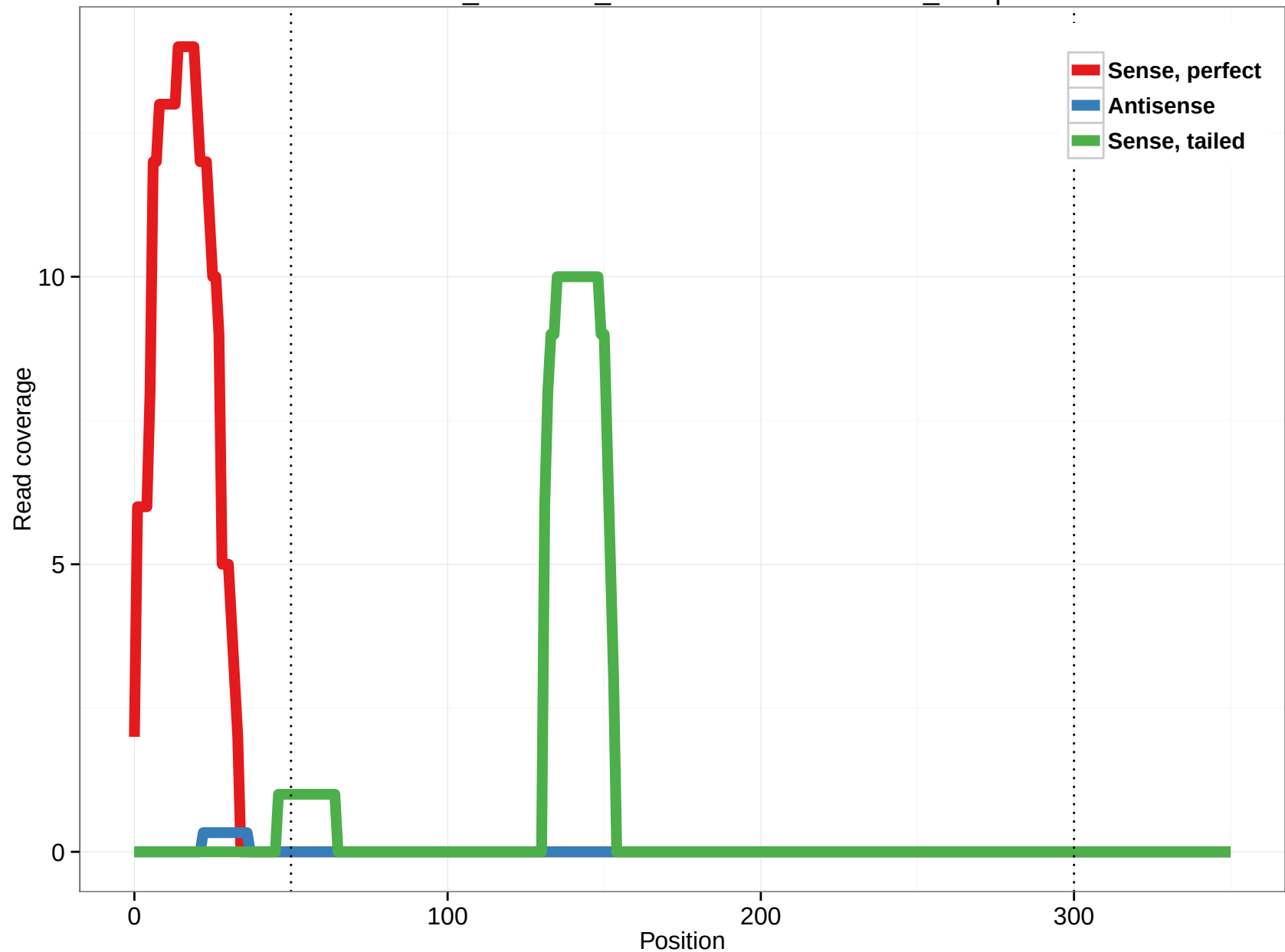
ornAna1_ensGene_ENSOANT00000000856_10.5p
