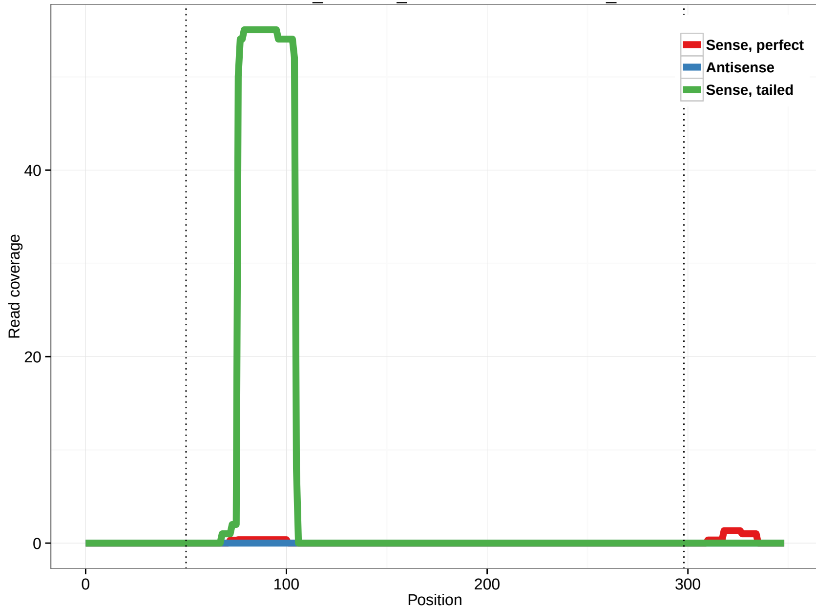
ornAna1_ensGene_ENSOANT00000000789_0
