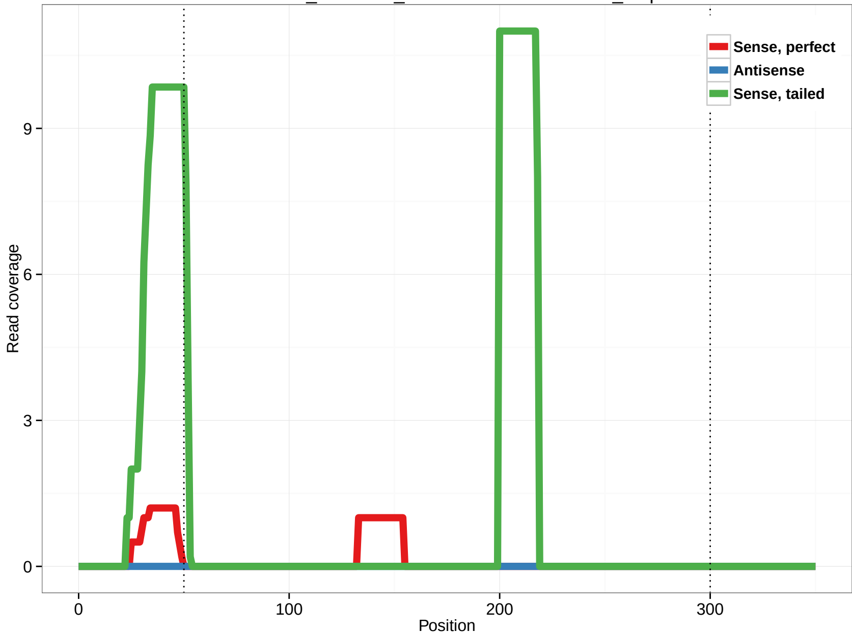
ornAna1_ensGene_ENSOANT00000000737_6.5p
