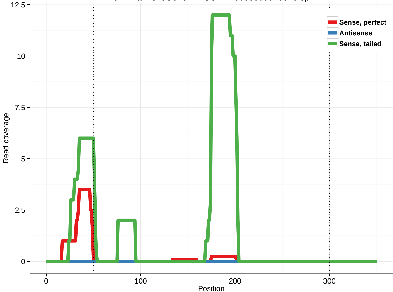
ornAna1_ensGene_ENSOANT00000000736_0.5p
