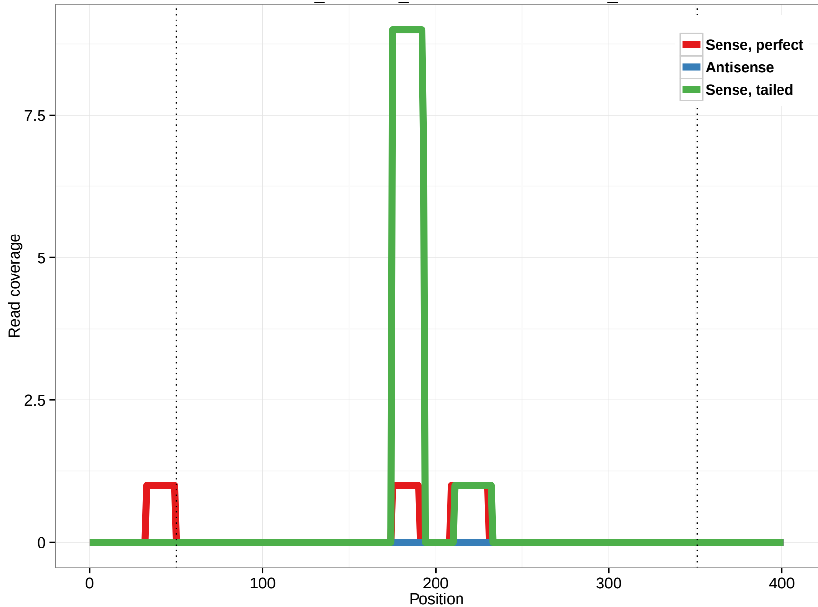
ornAna1_ensGene_ENSOANT00000000625_4
