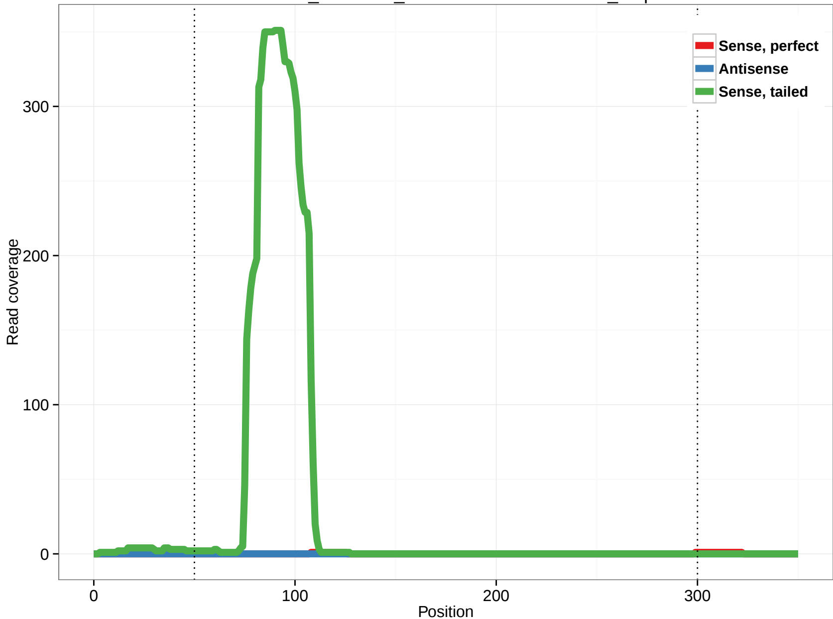
ornAna1_ensGene_ENSOANT00000000599_0.3p
