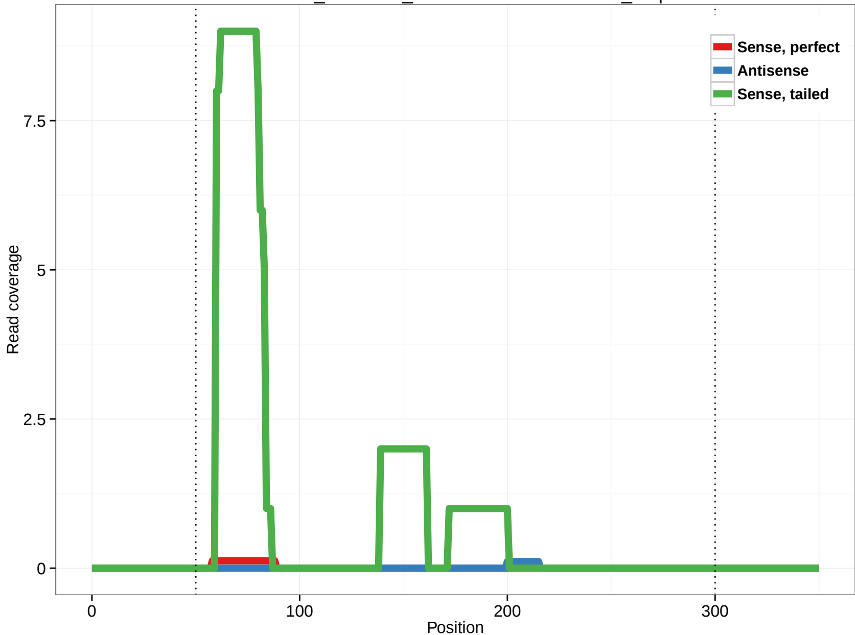
ornAna1_ensGene_ENSOANT00000000484_5.5p
