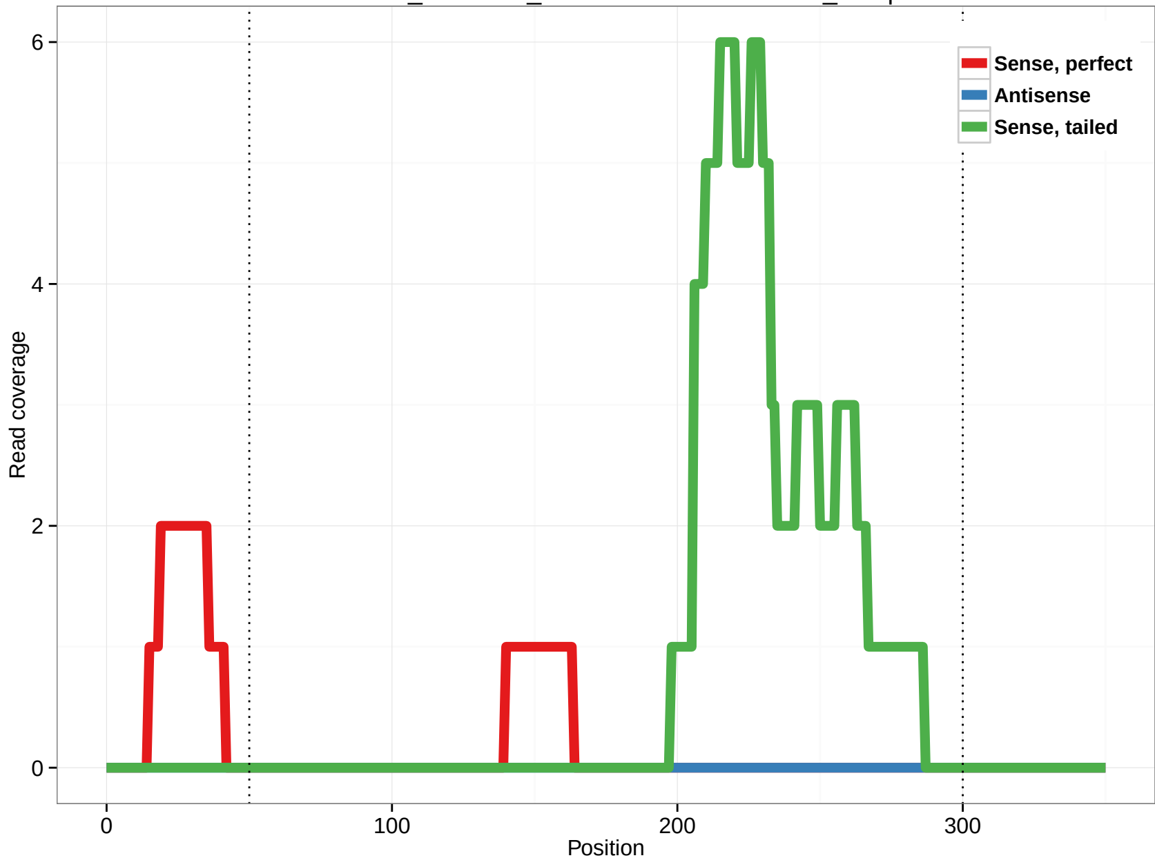
ornAna1_ensGene_ENSOANT00000000482_11.5p
