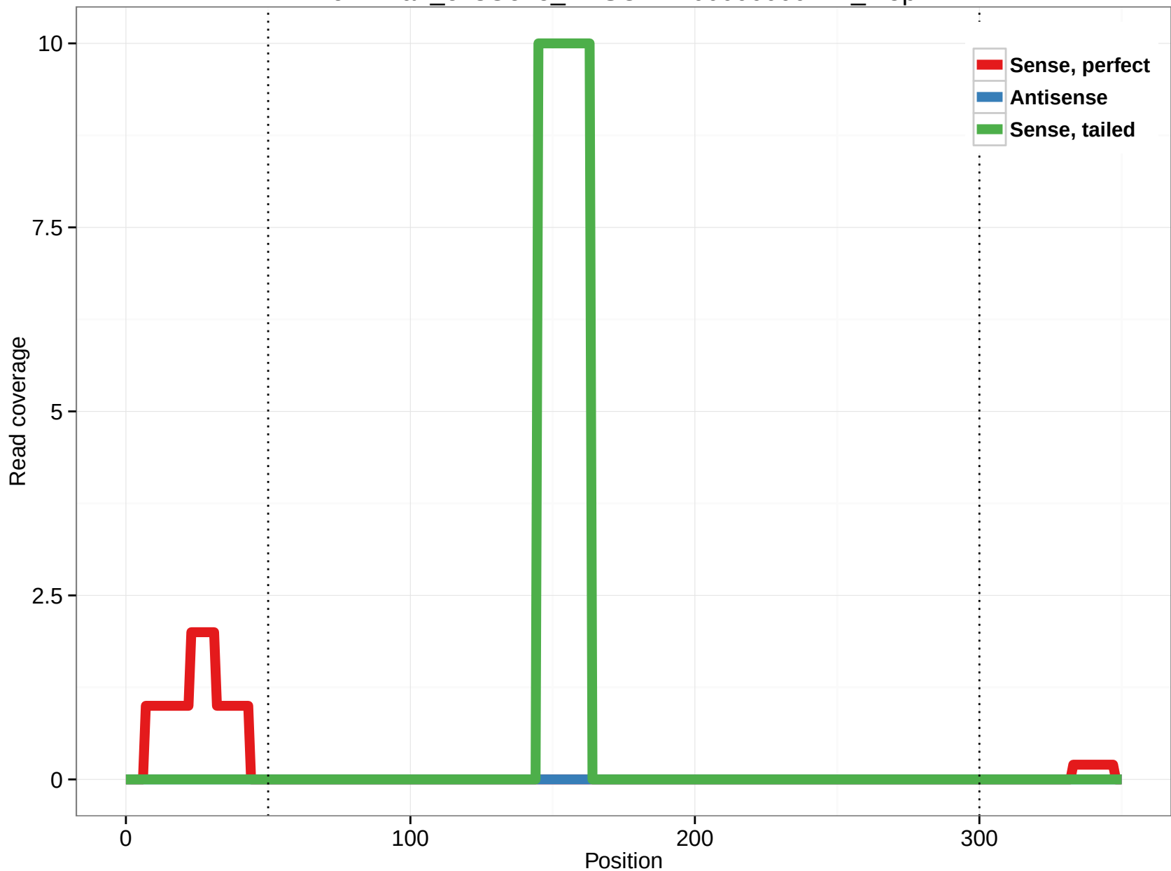
ornAna1_ensGene_ENSOANT00000000474_7.5p
