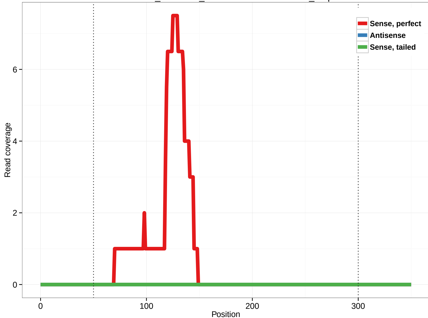
ornAna1_ensGene_ENSOANT00000000273_2.5p
