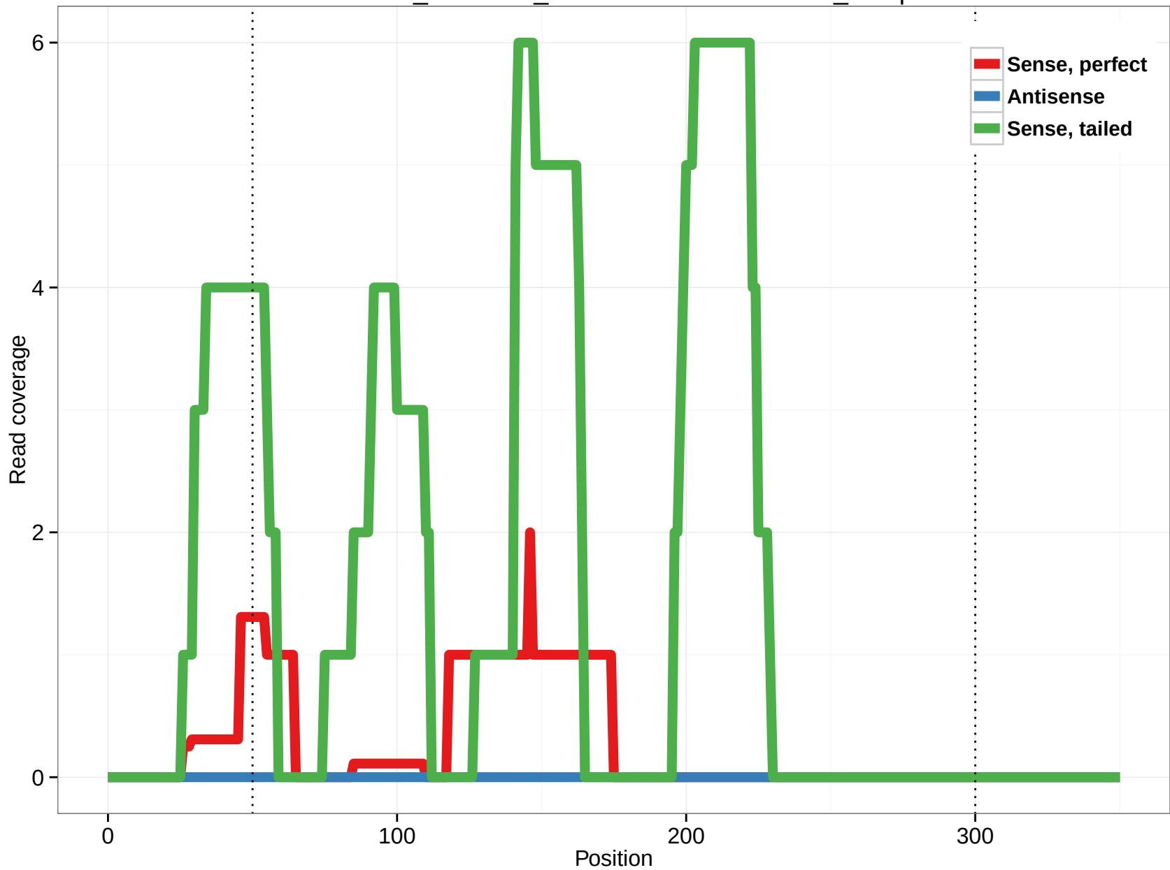
ornAna1_ensGene_ENSOANT00000000255_26.5p
