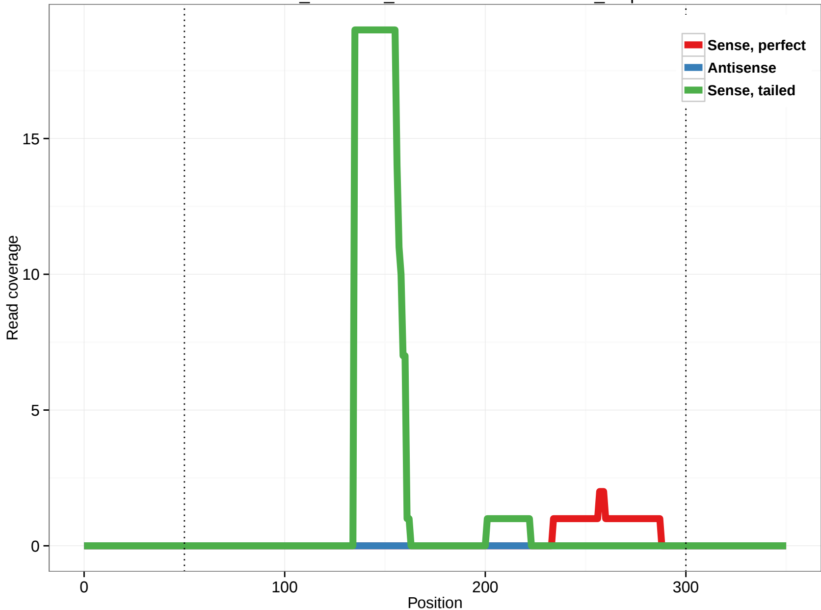
ornAna1_ensGene_ENSOANT00000000224_1.3p
