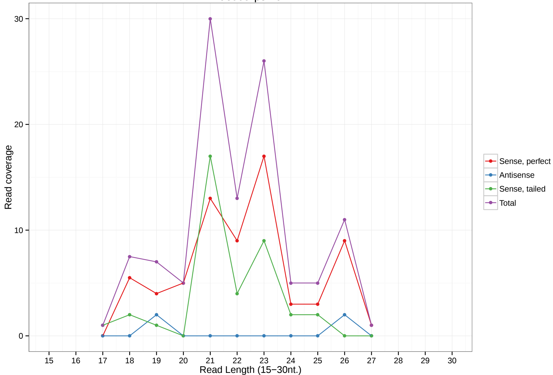
uc009rps.16
