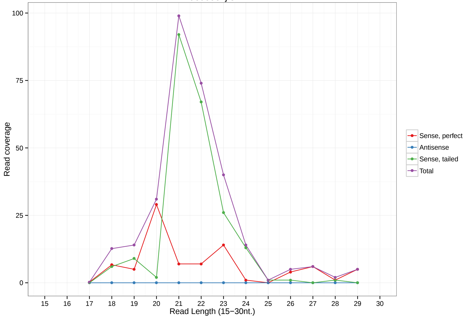
uc009cnj.5
