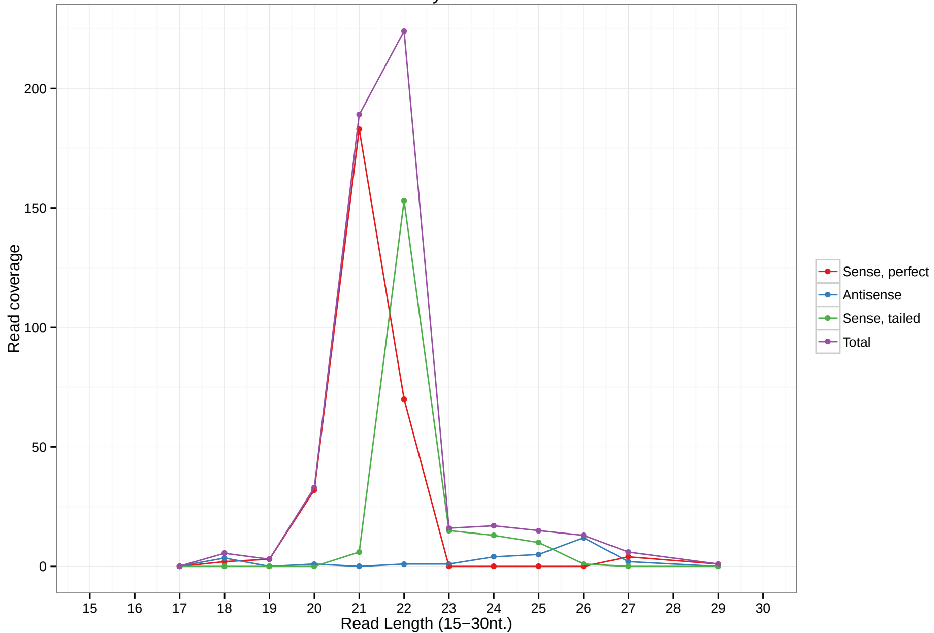
uc008ybl.0
