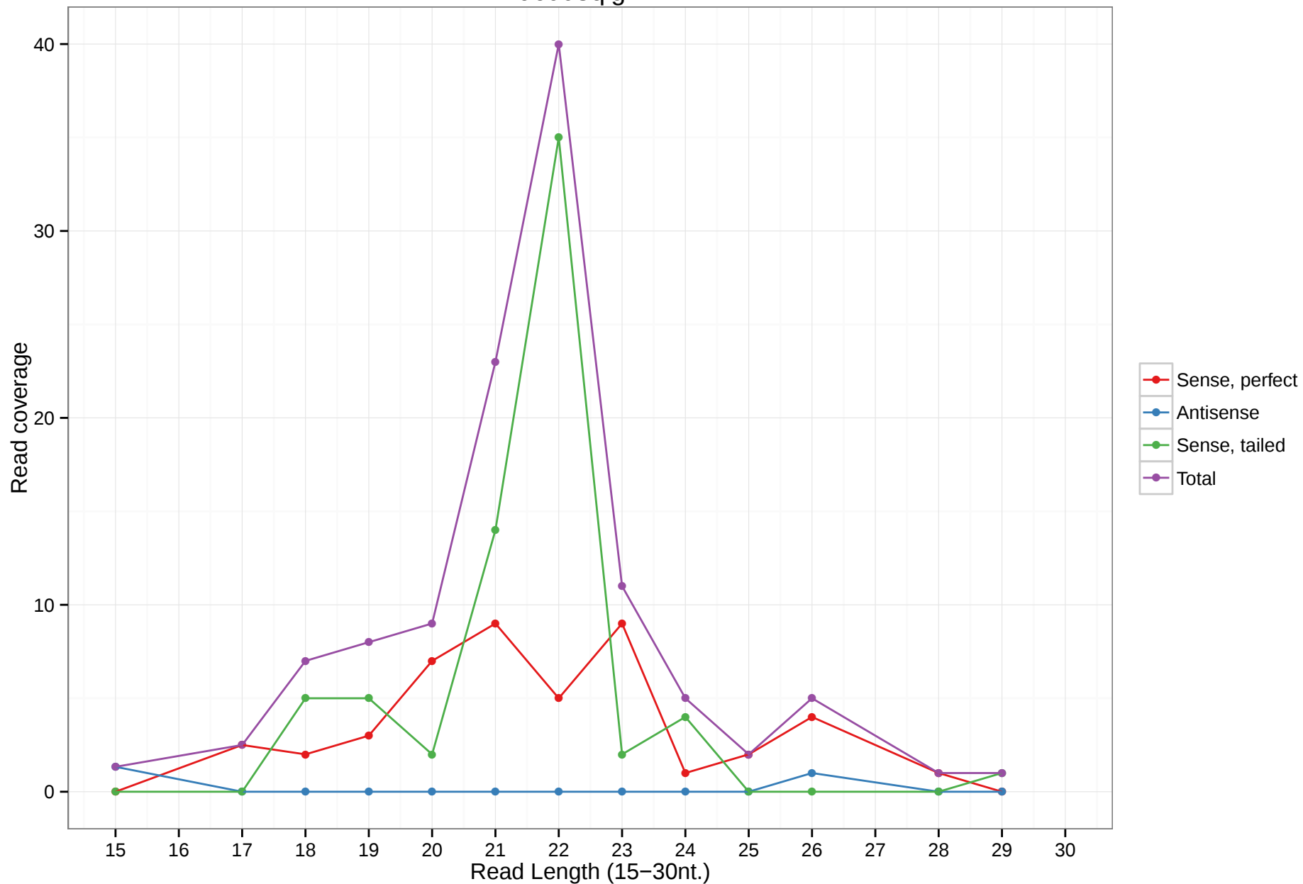
uc008qig.11
