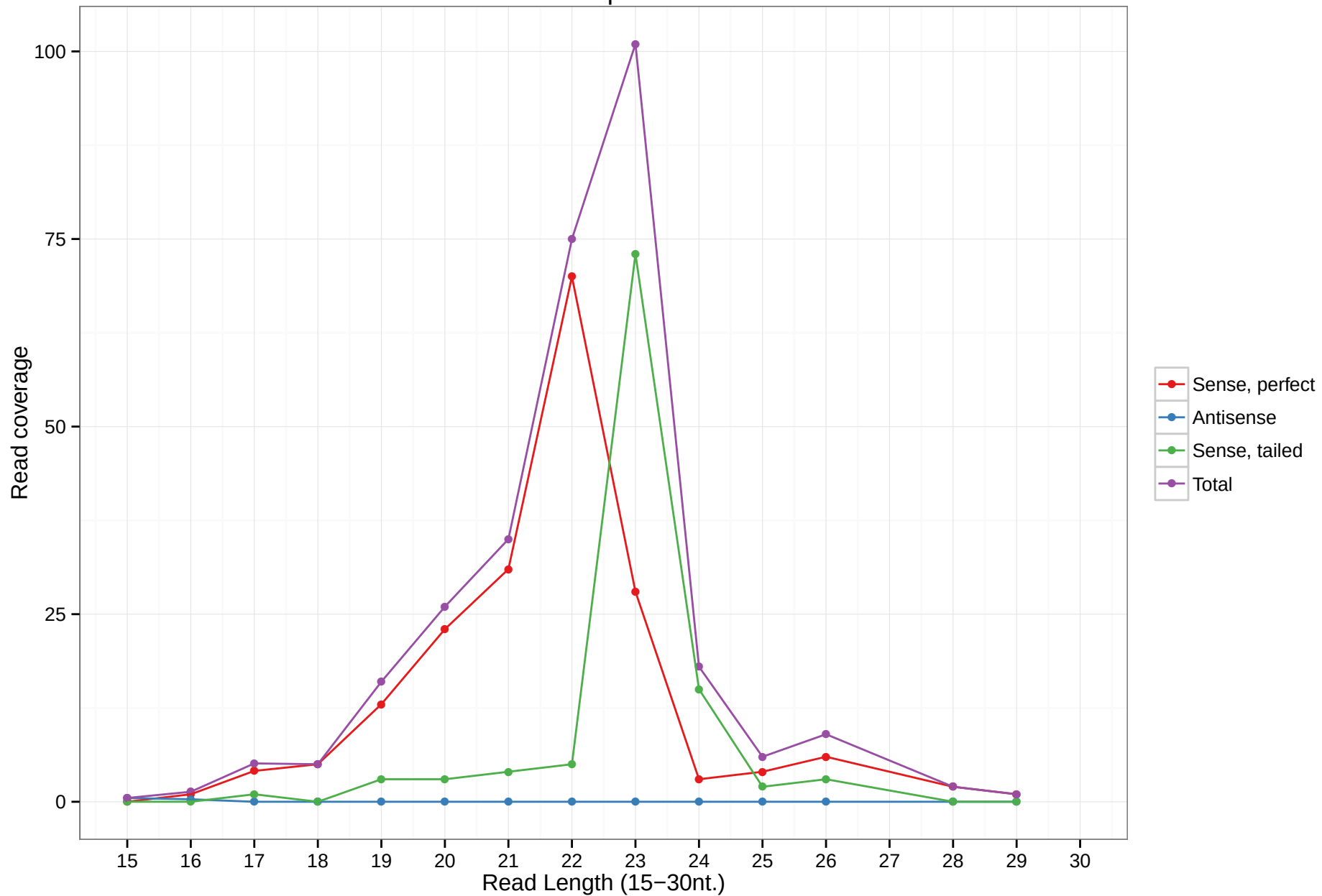
uc008pvu.3
