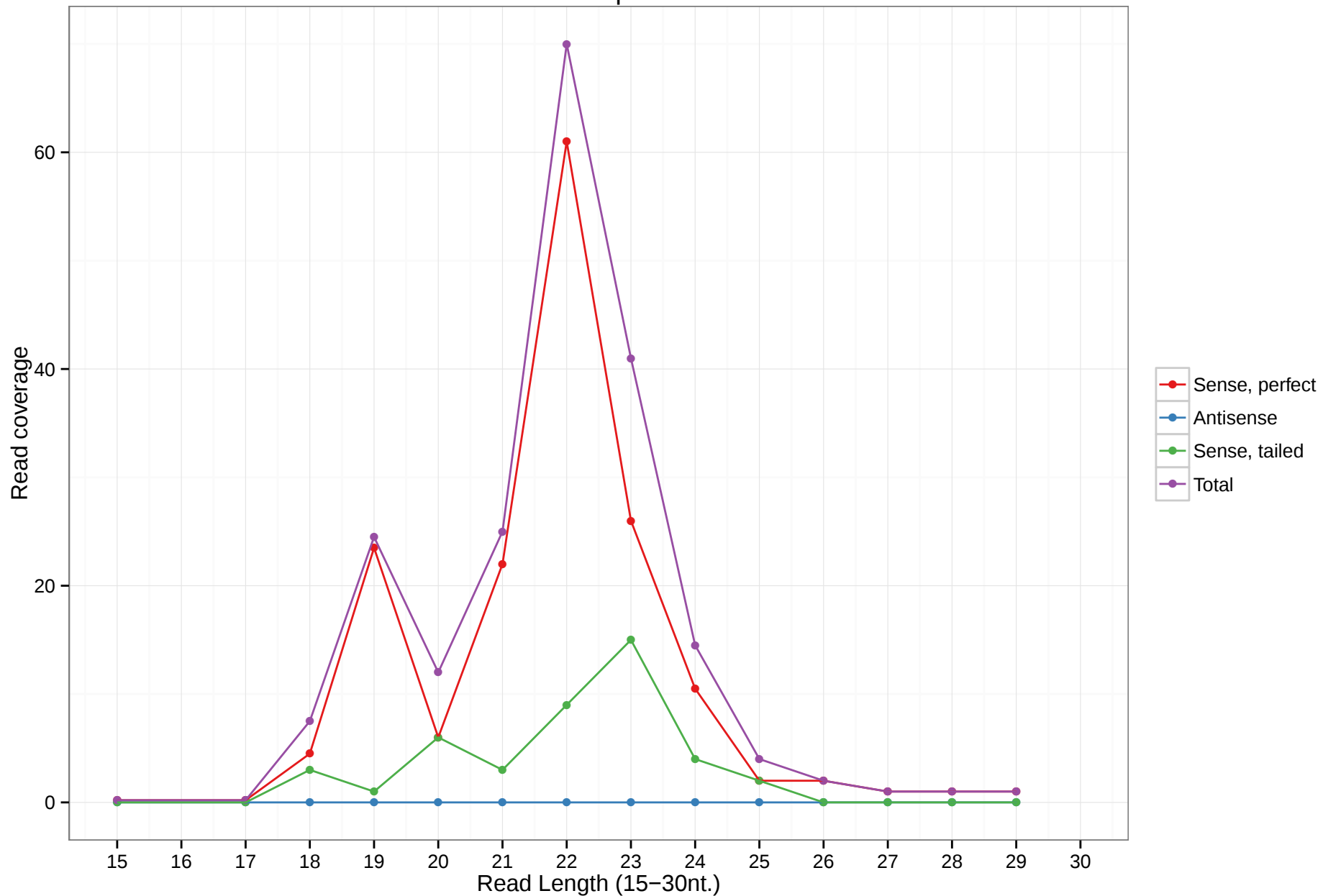
uc007qvf.7
