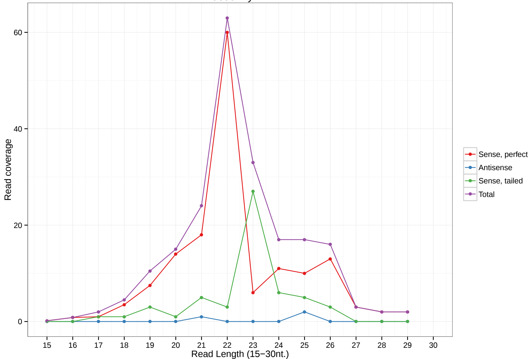
uc007iry.12
