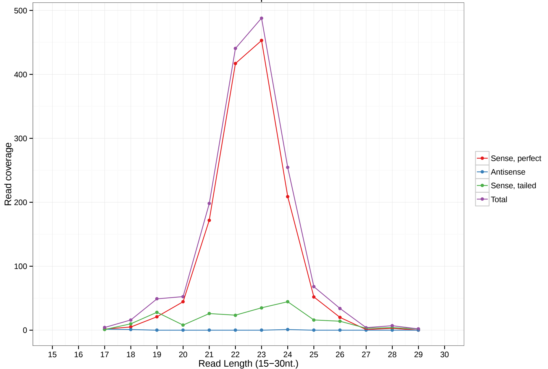
uc007ihp.3
