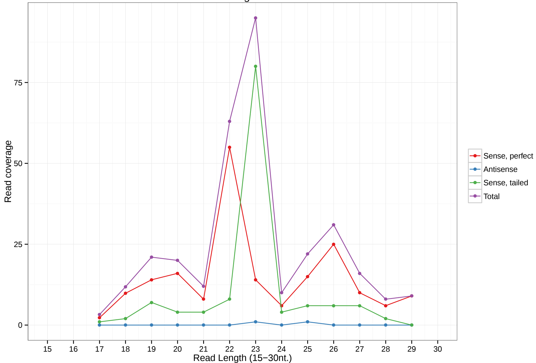
uc007gee.6
