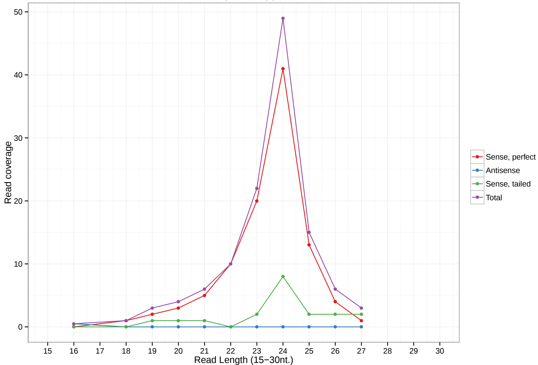
mmu-mir-7062
