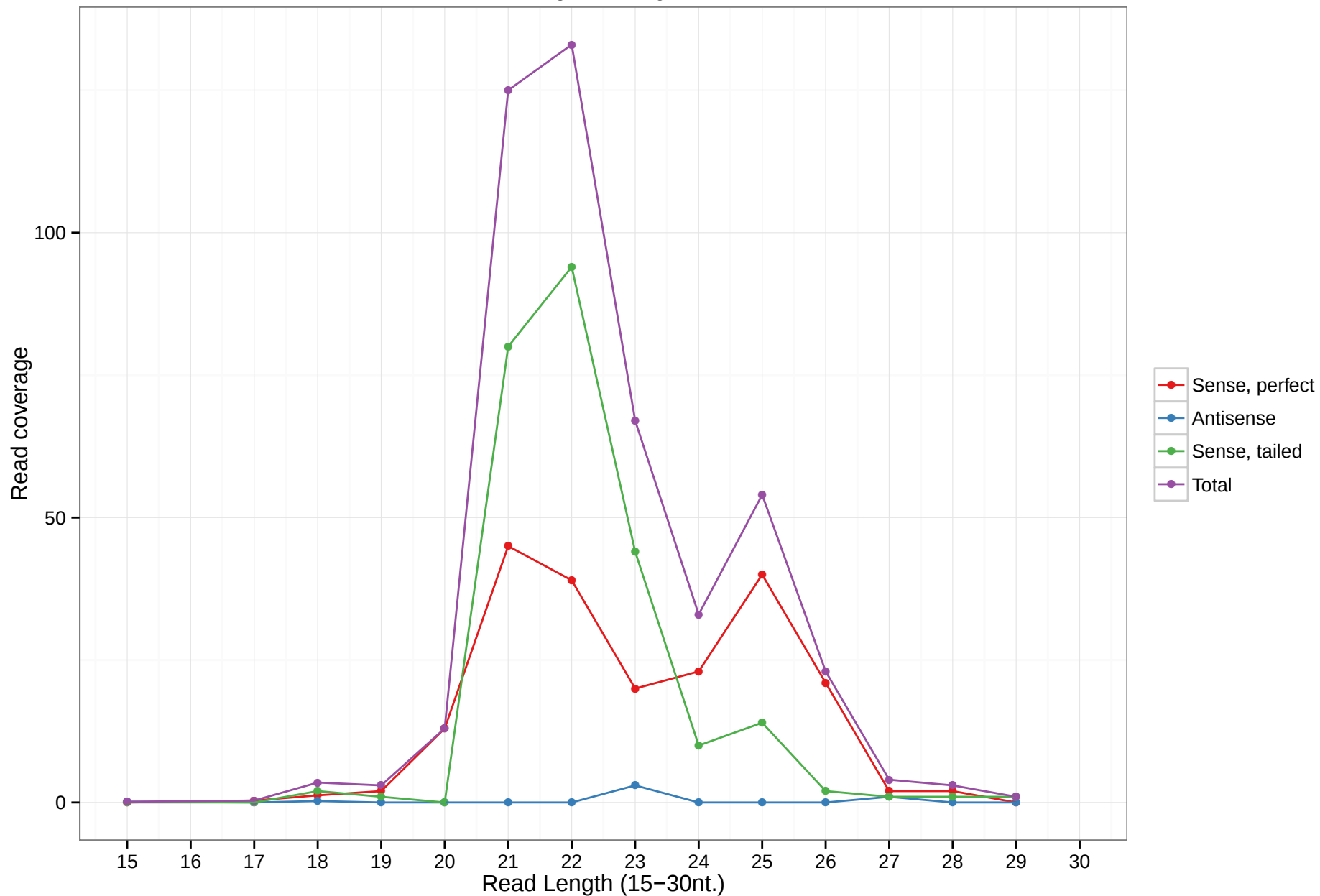
mmu-mir-7041
