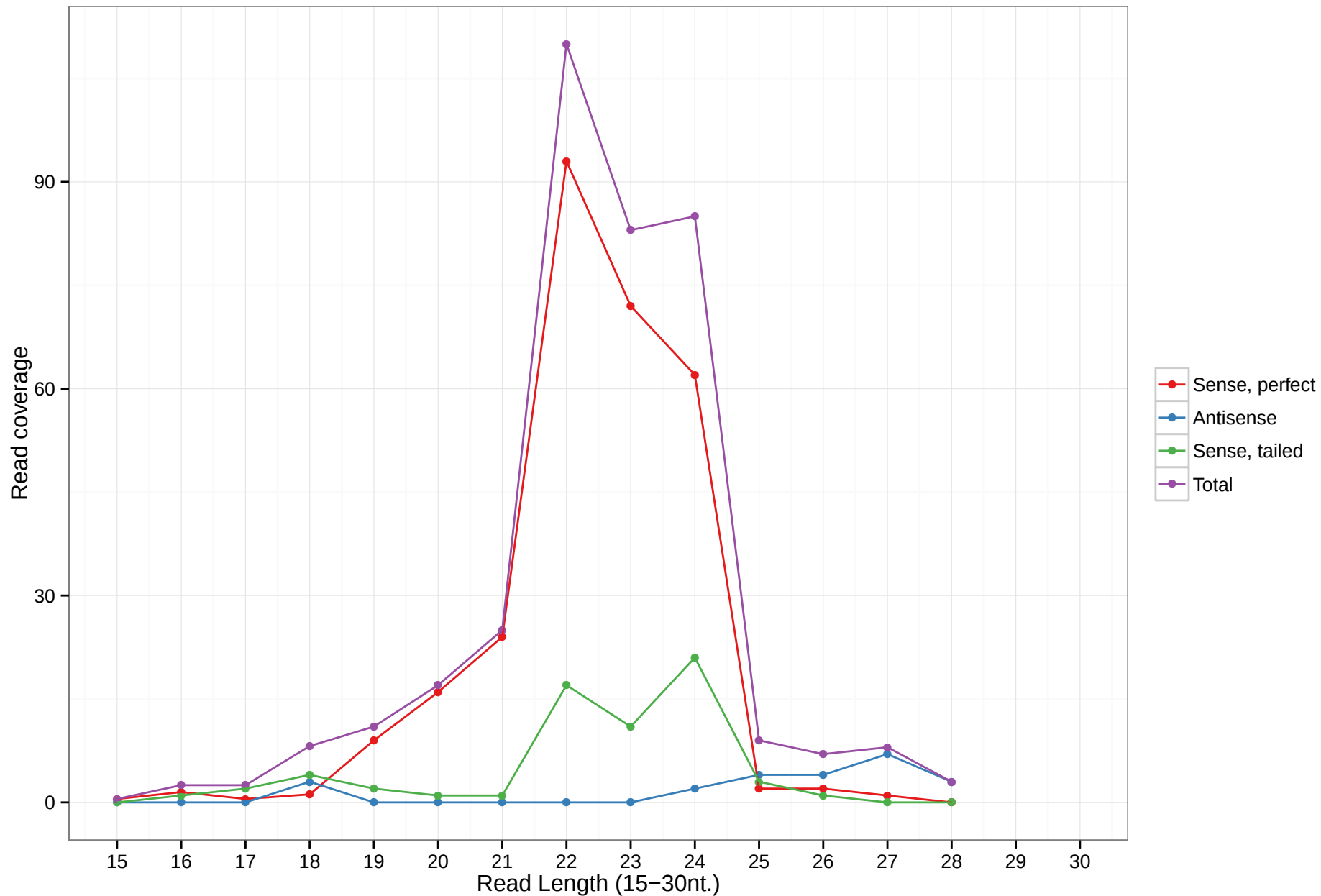
mmu-mir-6999
