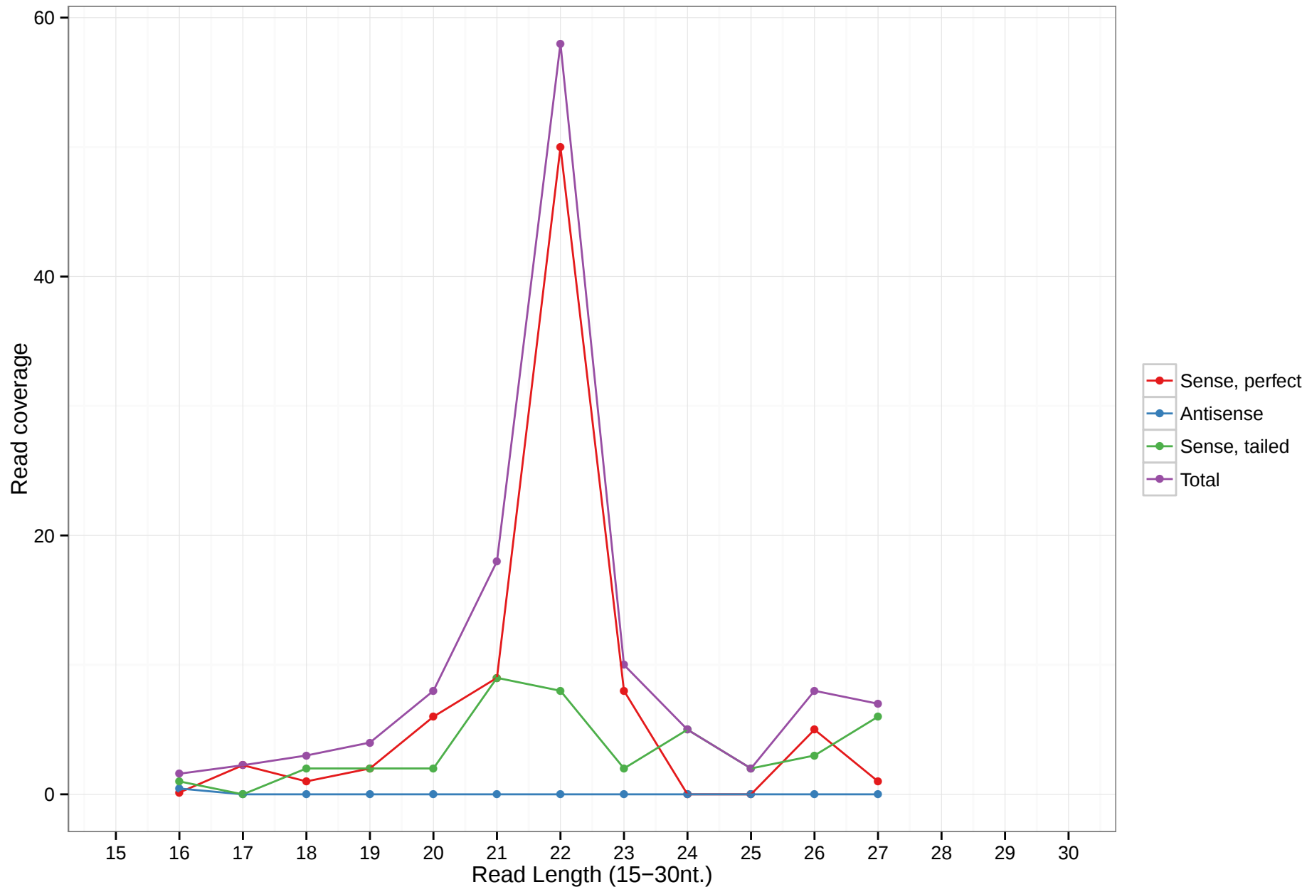
mmu-mir-6982
