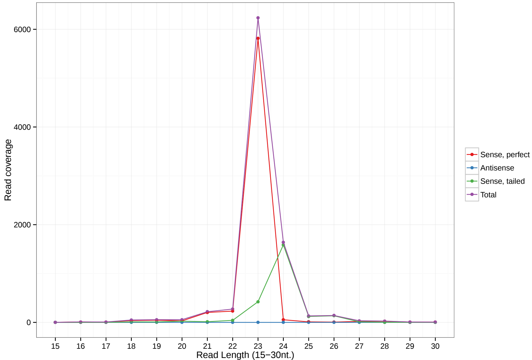
mmu-mir-6978
