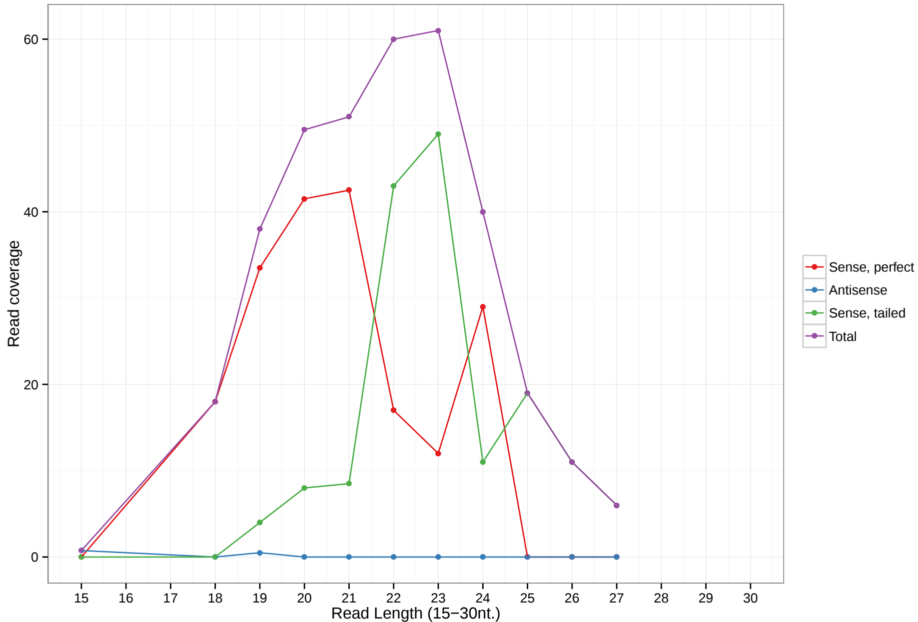
mmu-mir-6974
