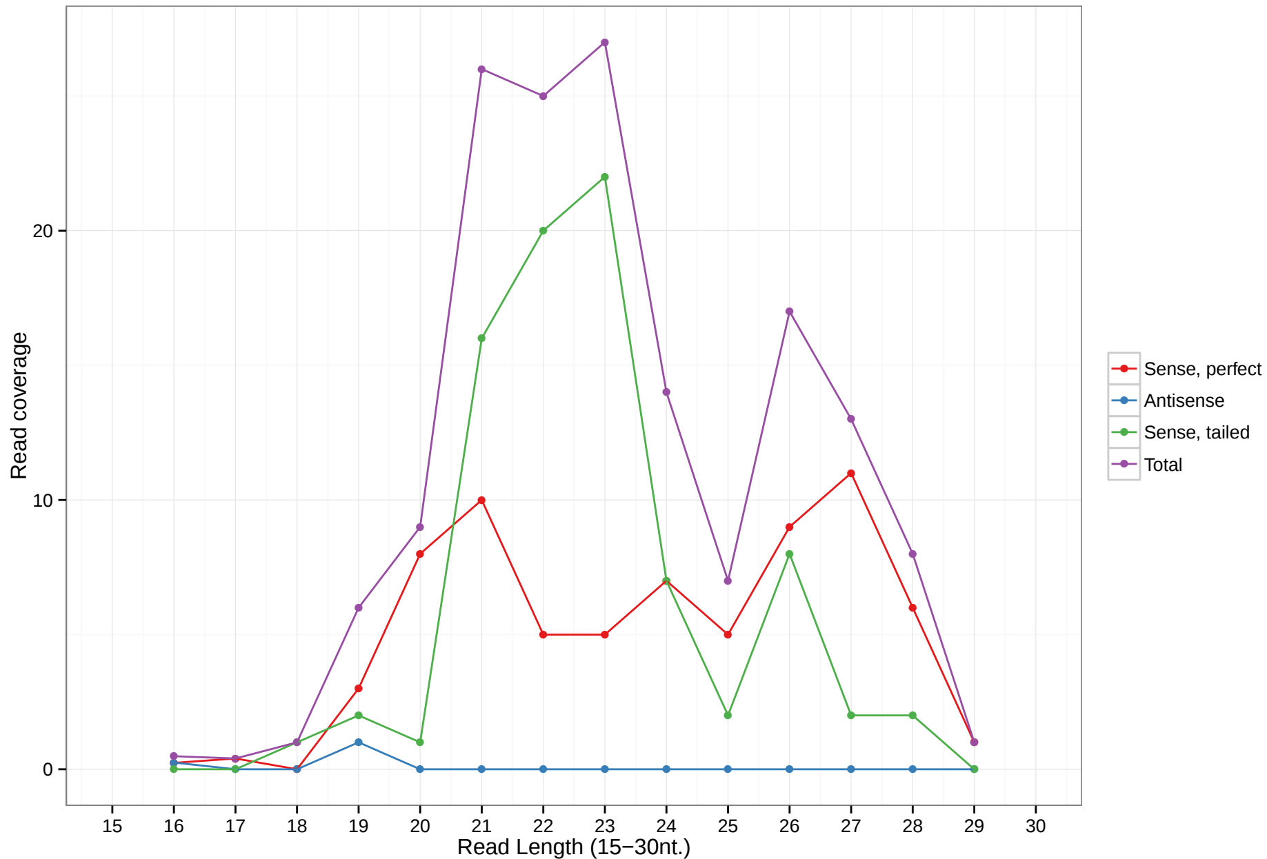
mmu-mir-6973b
