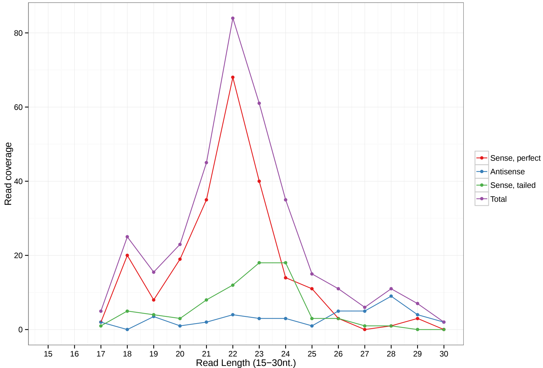
mmu-mir-6973a
