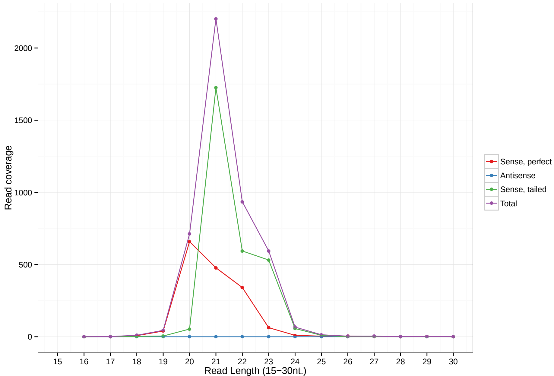
mmu-mir-6969
