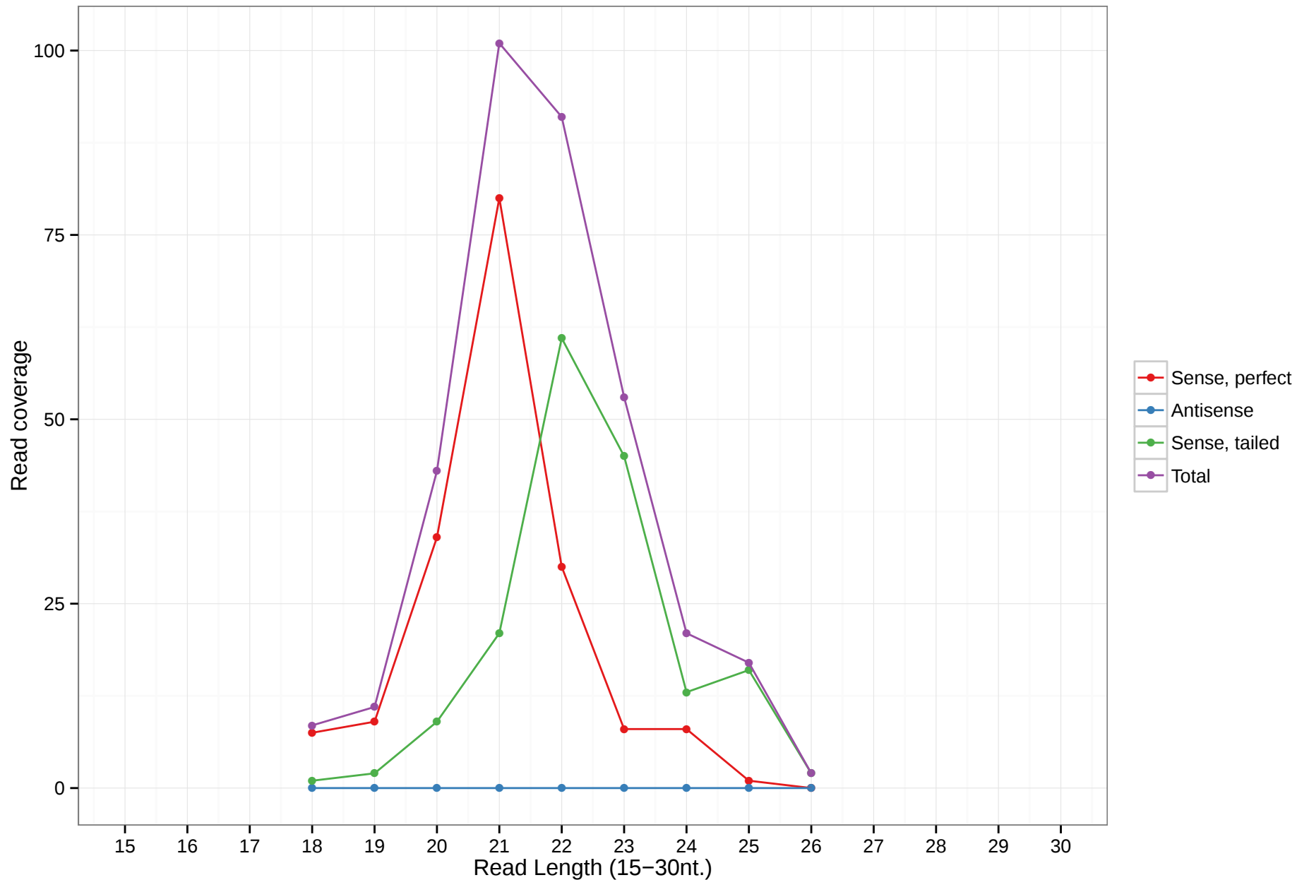
mmu-mir-6957
