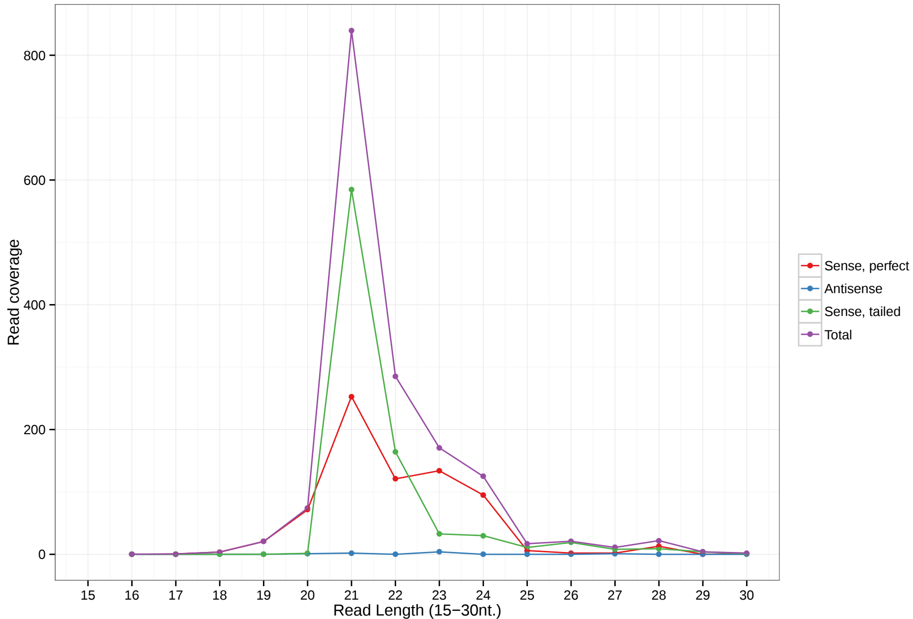
mmu-mir-6946
