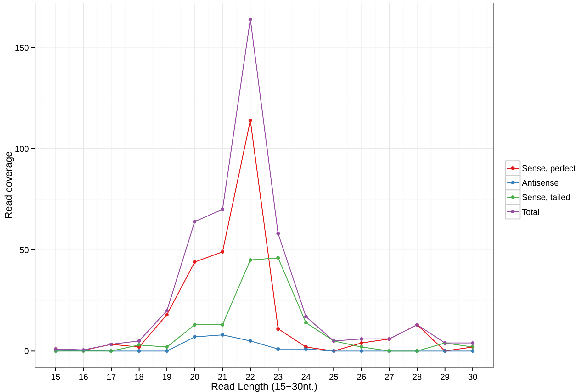
mmu-mir-6934
