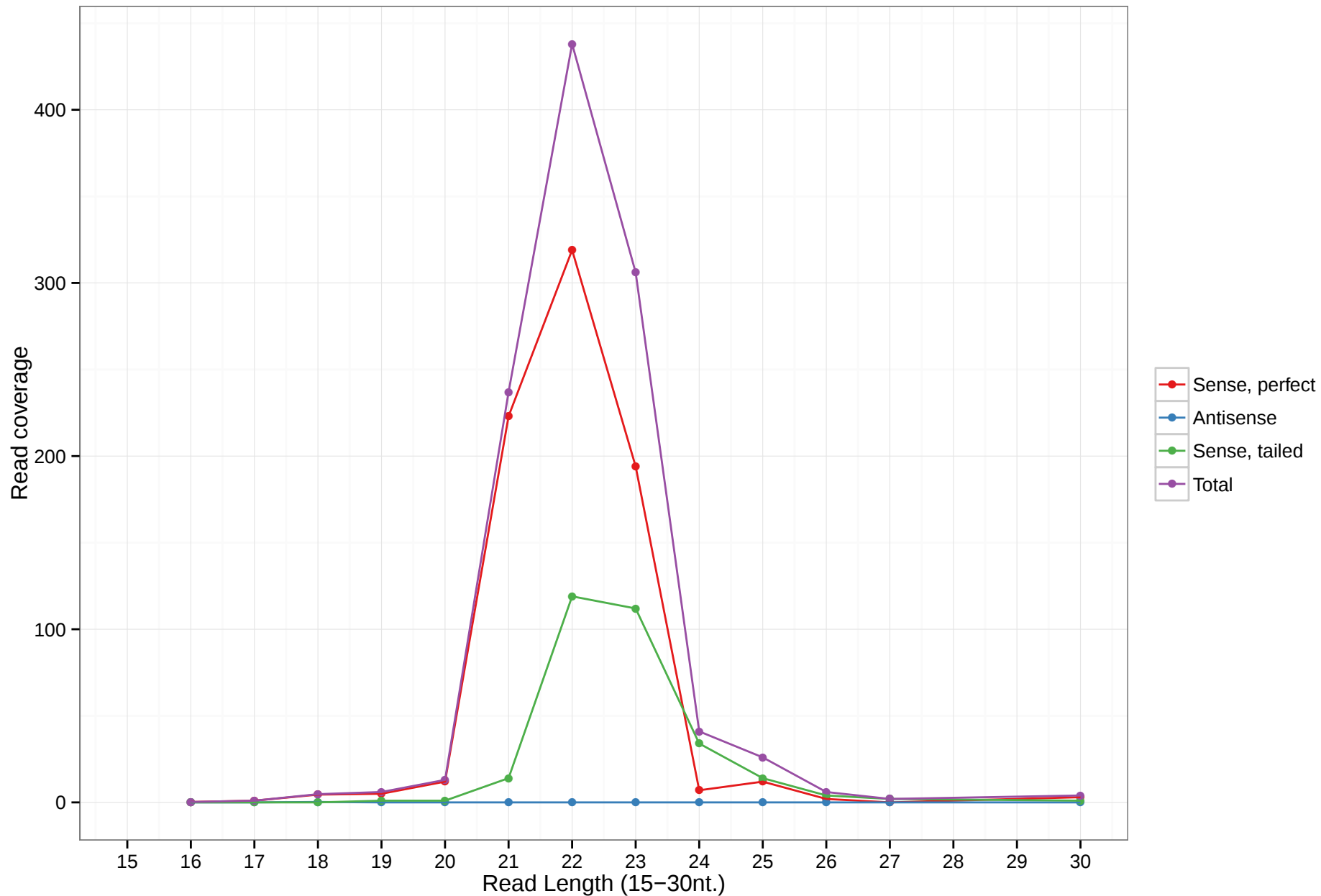
mmu-mir-6932
