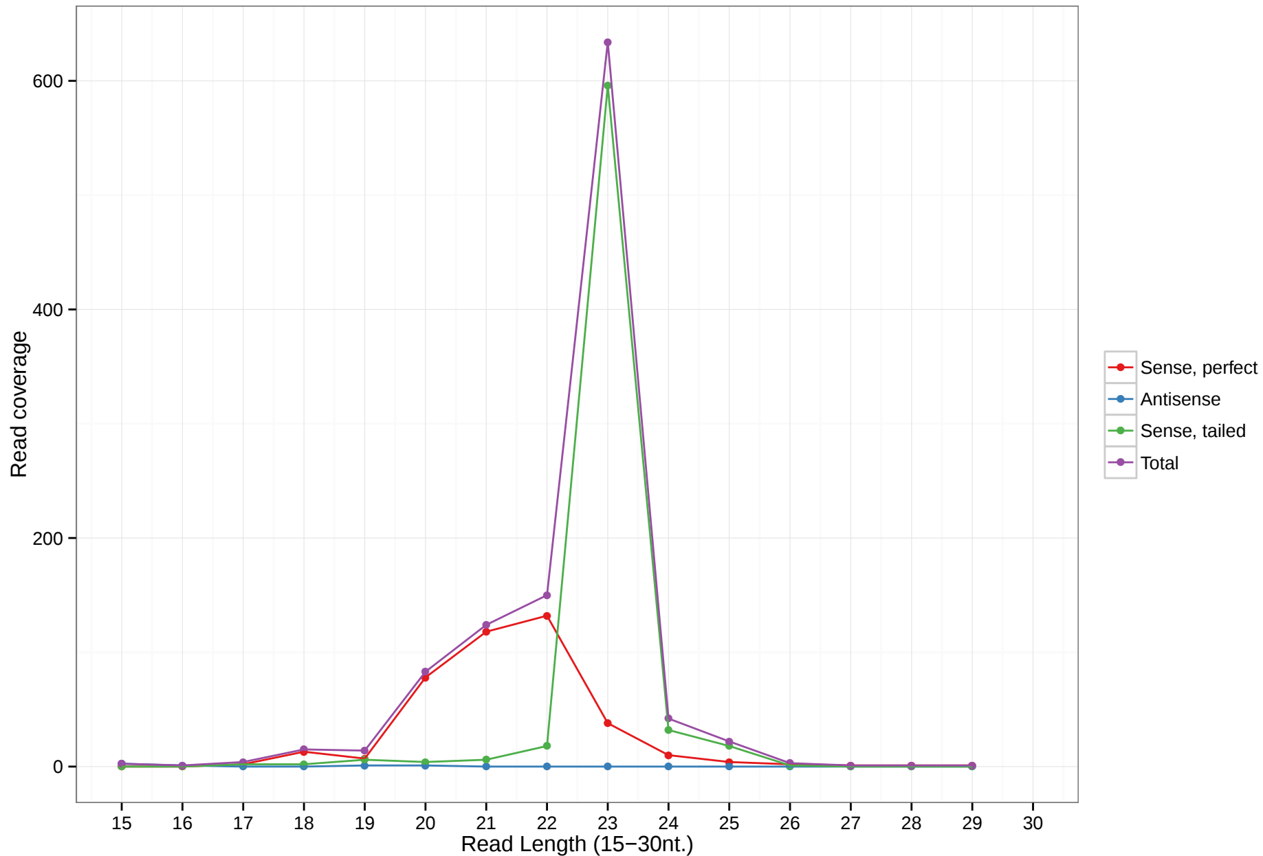
mmu-mir-6928
