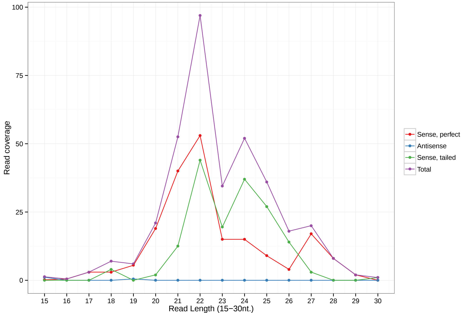
mmu-mir-6927
