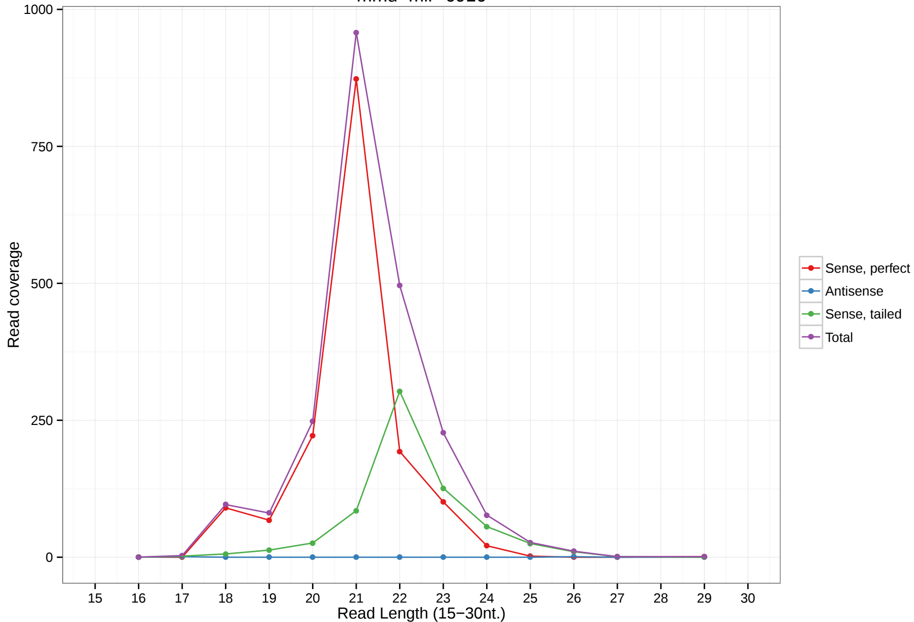
mmu-mir-6916
