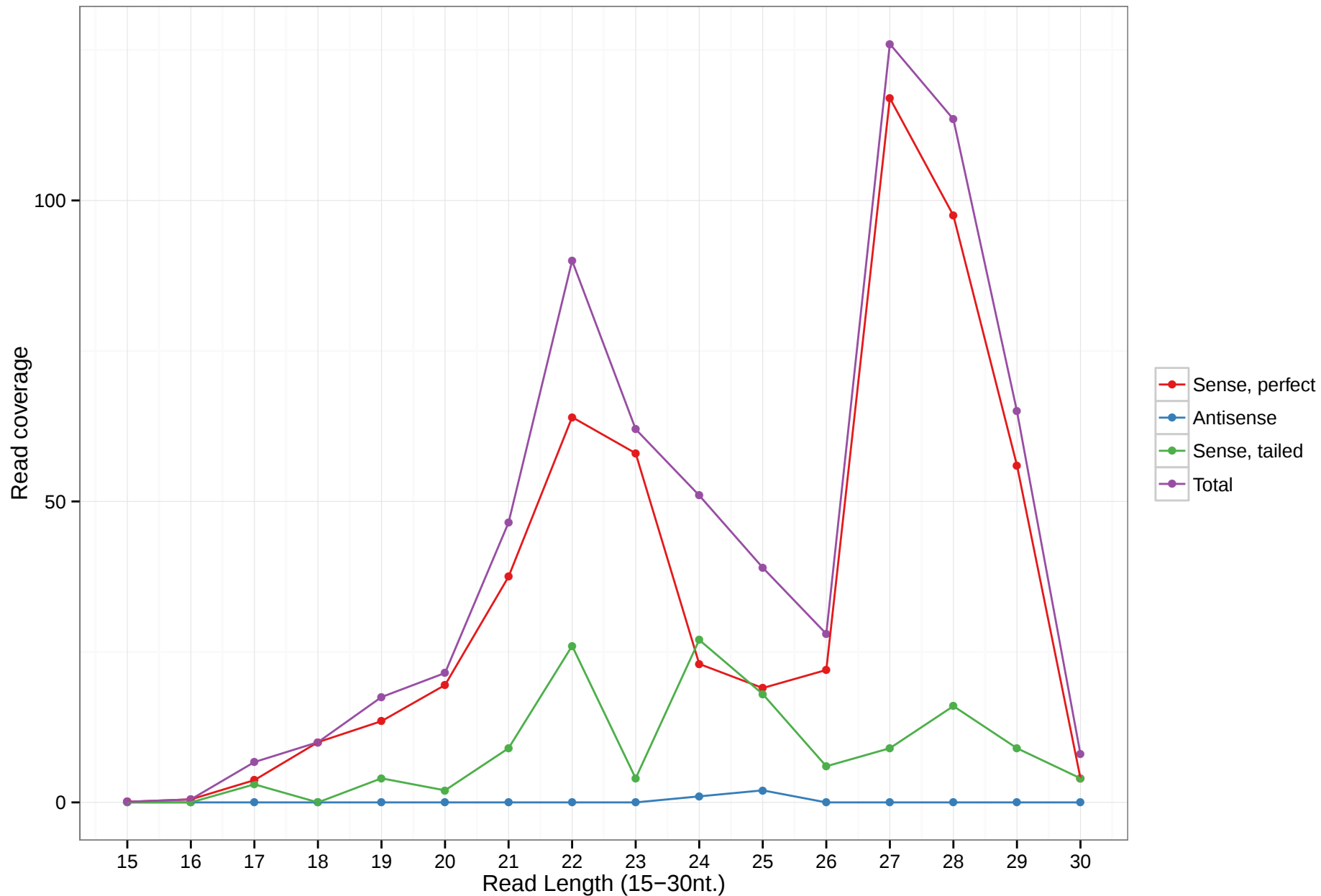
mmu-mir-6910
