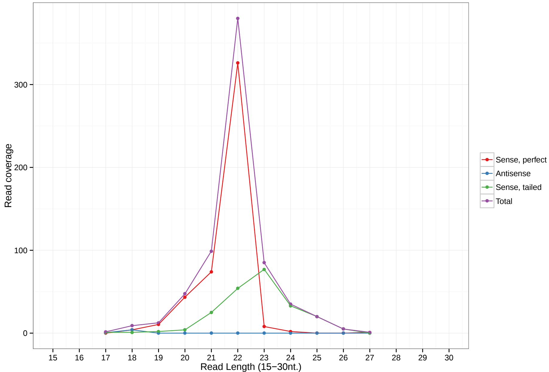
mmu-mir-6909
