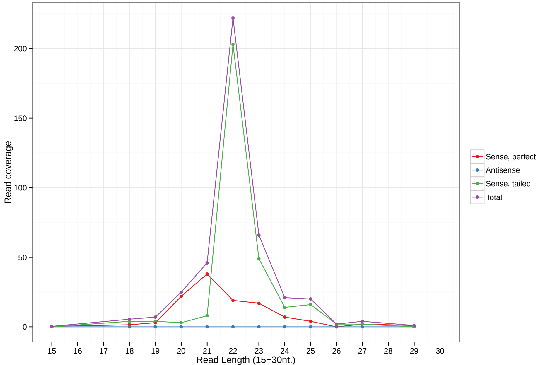
mmu-mir-6906
